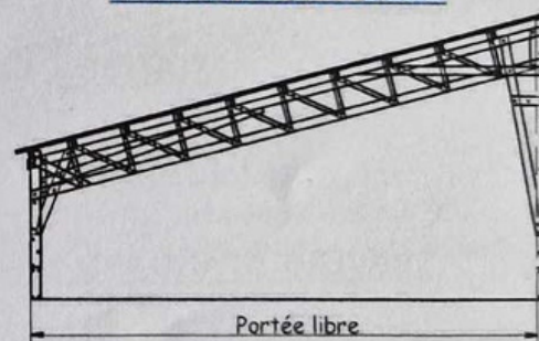
APPENTIS ACCOLES
