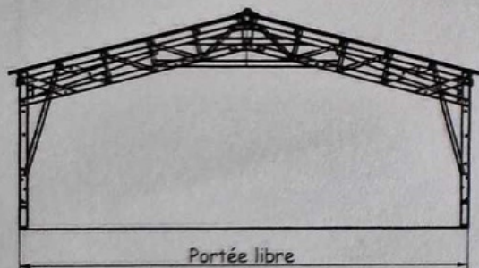
DOUBLES PENTES
